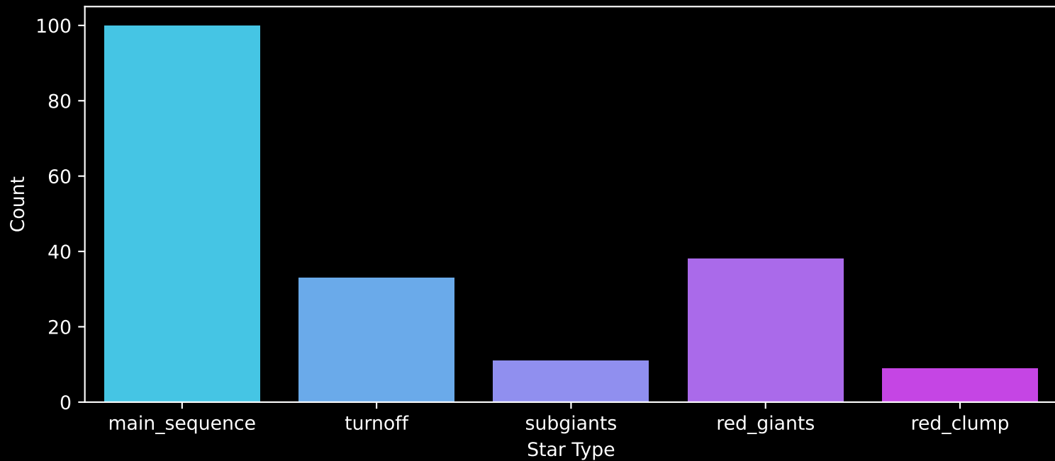
APOGEE DR17 Field: [198+41_MGA] Count plot of Star Type
