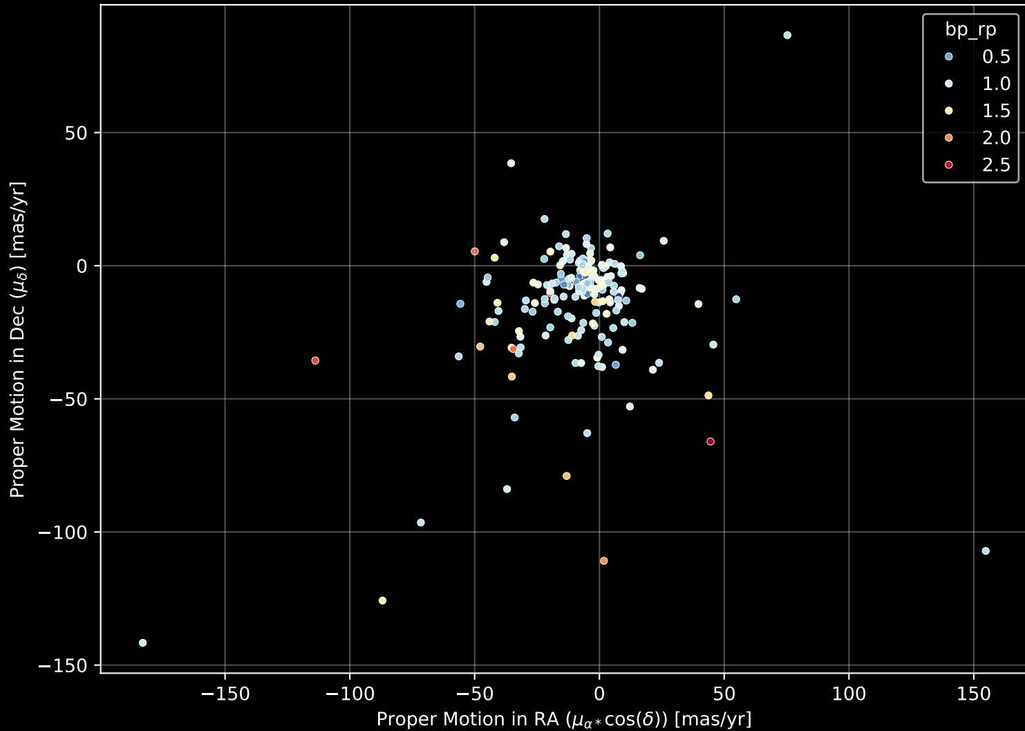
APOGEE DR17 Field: [198+41_MGA] Proper Motion Diagram (n= 191)
