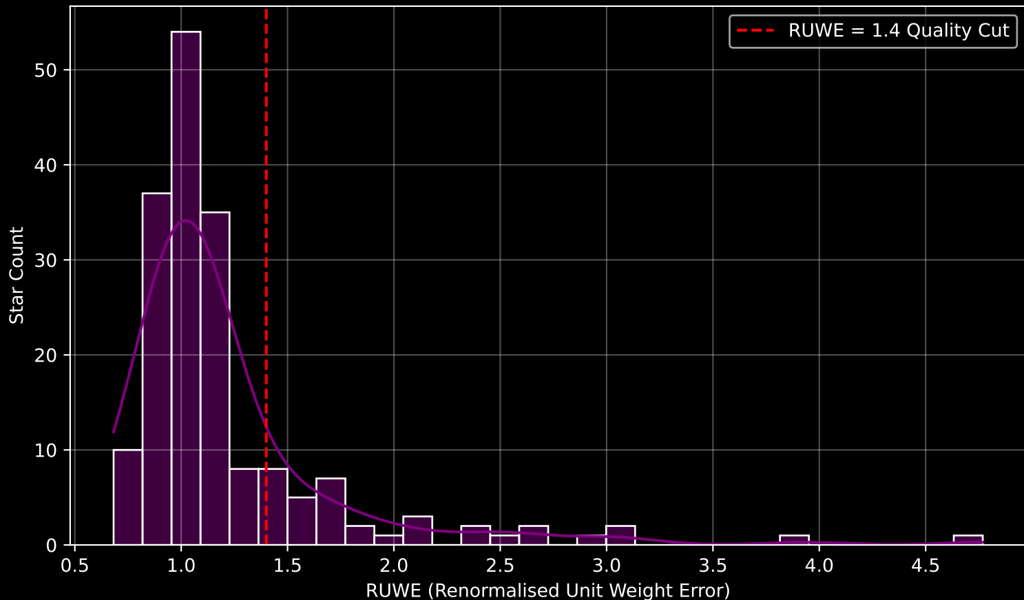
GAPOGEE DR17 Field [198+41_MGA] RUWE Distribution (n= 180)
