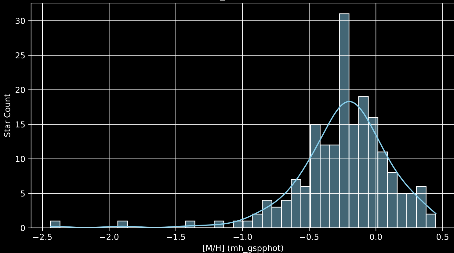
APOGEE DR17 Field: [198+41_MGA [M/H] (mh_gspphot) (n= 189)
