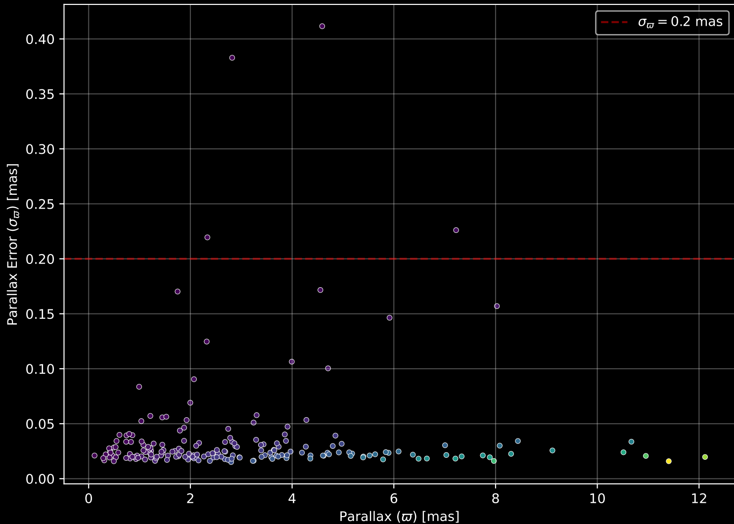
APOGEE DR17 Field: [198+41_MGA] Parallax Quality (n= 191)
